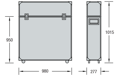
Q 510 Transport case for 1 basic module Q 400
