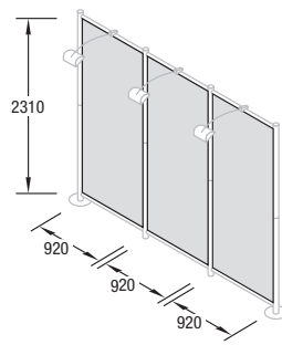
Q 11 Wall infill panel set "fabric", white, with inserted mounting profile weight: 8.38 lbs / 3.8 kg
