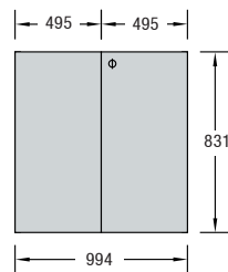
OL C580 Door set OCTALUMINA Counter
