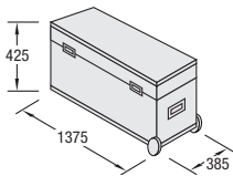
Q 501 Transport case for beams and accessories included in the corresponding sets
