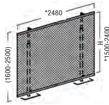
OP 100 Banner set straight 2 telescopic uprights and 4 beam extrusions 1240 mm long, incl. 2 base plates
