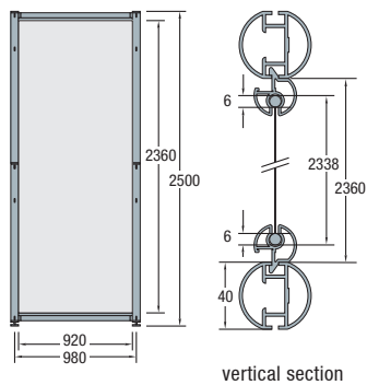
vertical section
