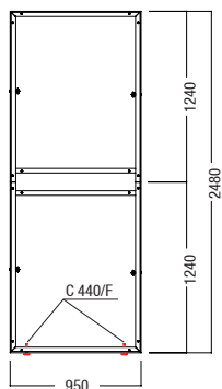
W 932 Frame, split incl. 2 adjustable feet
