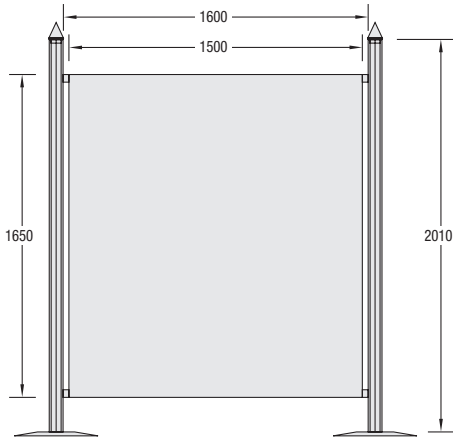
M 1350 Banner set, straight, 2 uprights, 80 mm dia., h=2010 mm, 2 beams 1600 mm long, incl. base plate and cone
