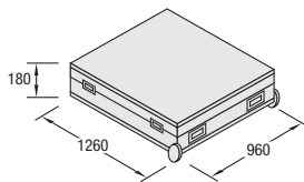
Q 503 Transport case for 3.2 mm wood wall panels and accessories included in wall infill panel set Q 42
