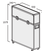
Q 504 Transport box with handle and castors, plastic / aluminium
