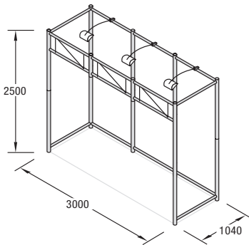
Q 20 Construction set incl. 2 transport cases Q 502 and lighting 230 V weight: 120.15 lbs / 54.5 kg
