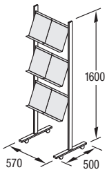
P-6 6 acrylic shelves with castors
