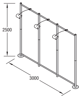
Q 10 Construction set incl. cardboard box and lighting 230 V weight: 70.55 lbs / 32.0 kg
