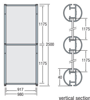
vertical section
