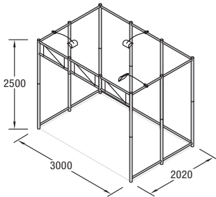
Q 30 Construction set incl. 2 transport cases Q 502 and lighting 230 V weight: 147.71 lbs / 67.0 kg
