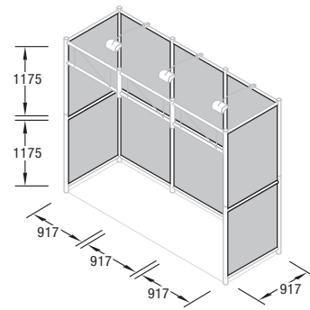
Q 22 Wall infill panel set, white, 3.2 mm, incl. 5 beams and wooden case weight: 85.98 lbs / 39.0 kg
