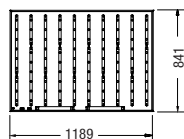
OL 400 Frame 40 mm, single-sided illuminated size: DIN A0 incl. 2 m cable and plug, power supply unit integrated, without graphics
