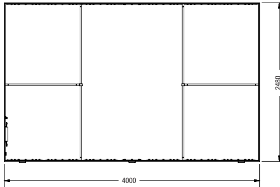
OL 1240 Frame 120 mm, double-sided illuminated, incl. 3 base plates, 2 m cable and plug, without graphics
