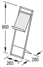
P-1 1 acrylic shelf
