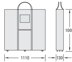
Q 511/N Transport bag with castors for 1 basic module Q 400 and 1 door set Q 411, grey
