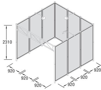
Q 41 Wall infill panel set "fabric", white, with inserted mounting profile weight: 23.35 lbs / 11.5 kg
