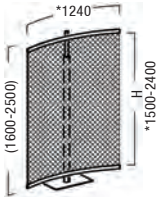
OP 20 Banner set curved concave 1 telescopic upright and 2 beam extrusions 1240 mm long, incl. 1 base plate
